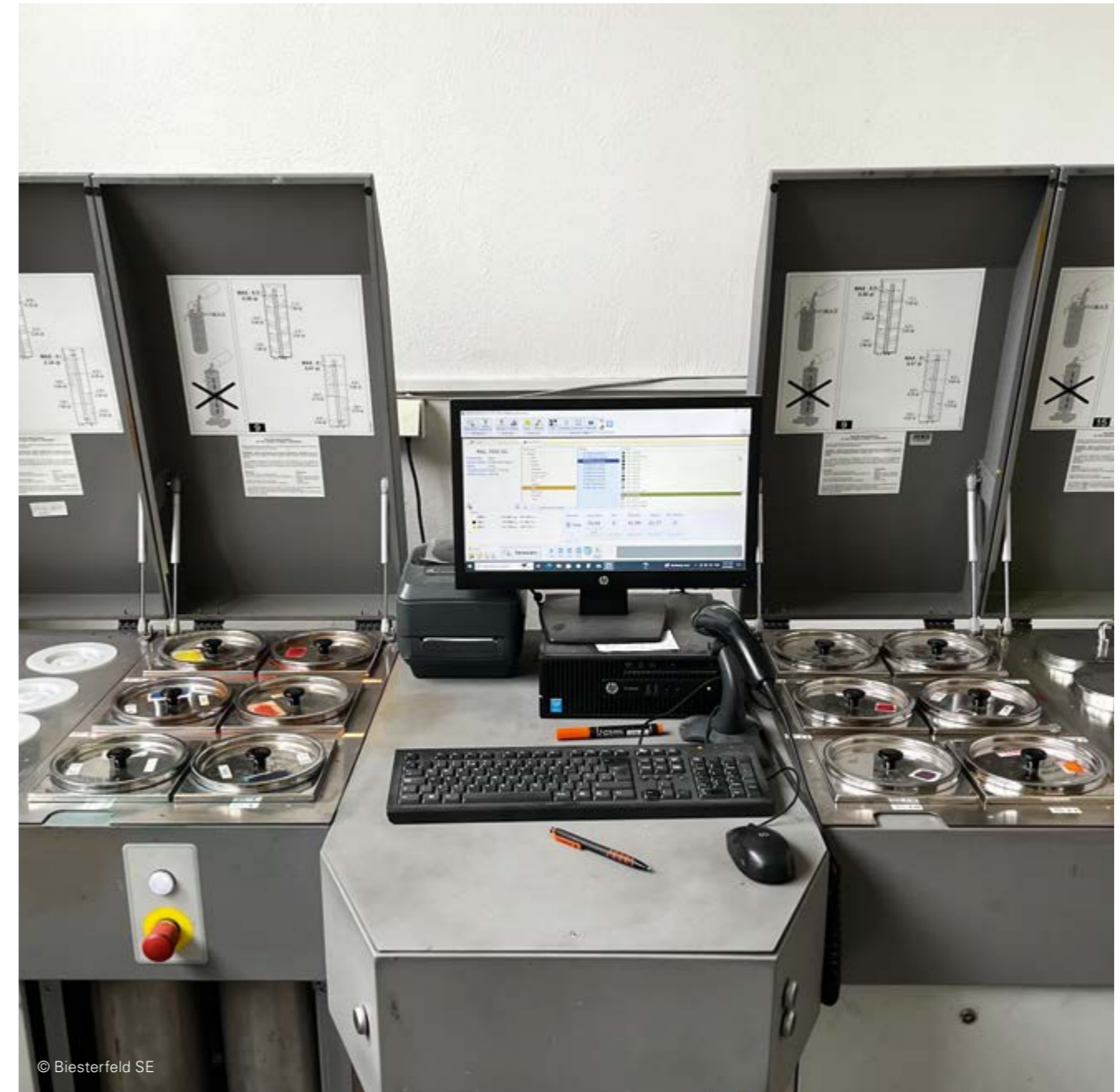
Scott Bader GelTint machine for customizing the colors of your gelcoats.
