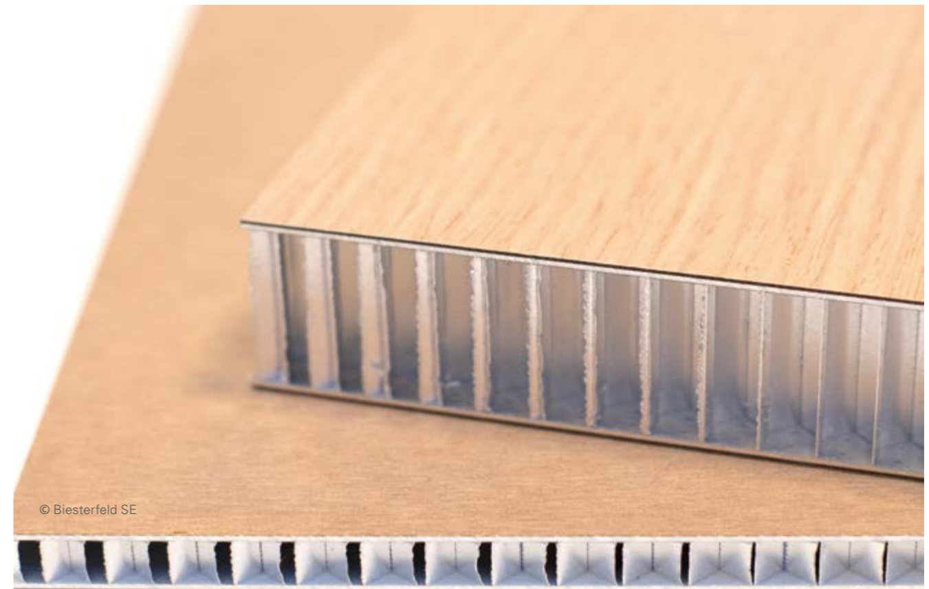
A close-up of aluminum honeycomb showcases its lightweight structure and exceptional strength, delivering optimal performance for advanced composite designs.
